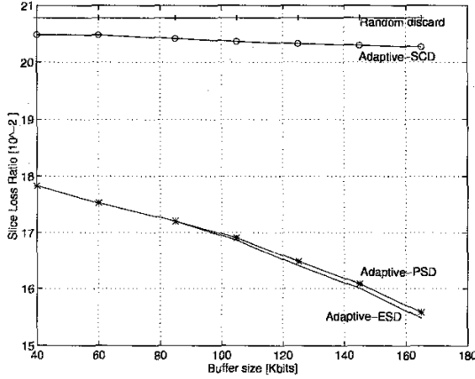
Figure 2 - (I) Intra-frame Slice Loss Ratio
