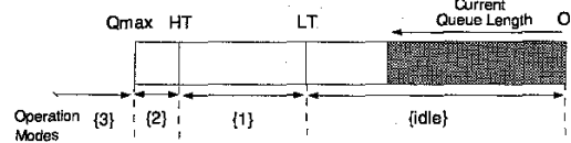
Figure 1 - Adaptive-PSD and Adaptive-ESD Operation Modes
