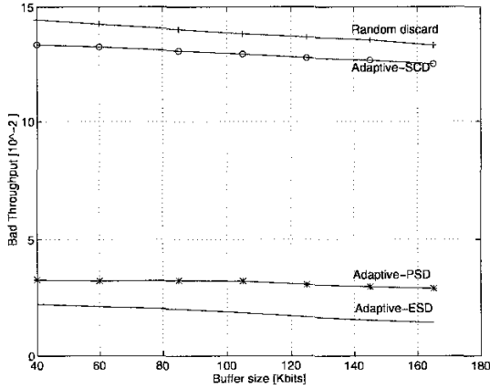
Figure 6 - Cell Bad Throughput
