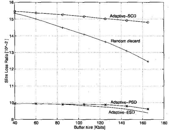
Figure 4 - (B) Bidirectional Predictive-frame Slice Loss Ratio
