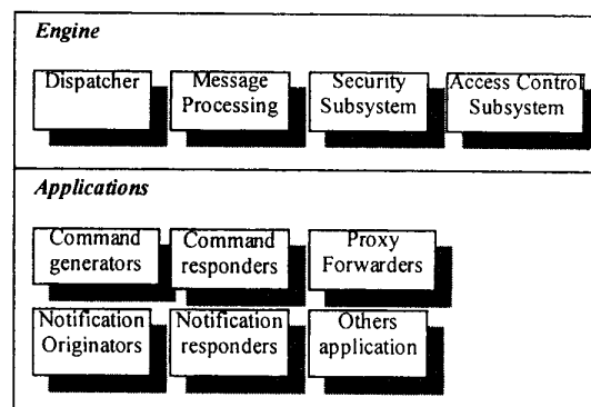
Figure 1: Architecture of SNMPv3 entities
