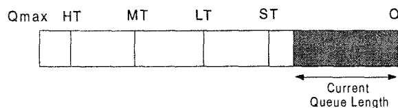
Figure 5 - Switch Buffer thresholds
