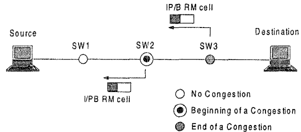
Figure 1 - Transmission of I/PB RM cells
