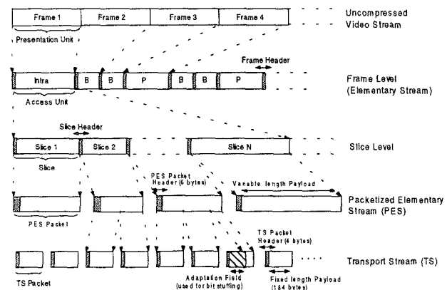
Figure 3 - Slice-based PES Encapsulation using variable length packet
