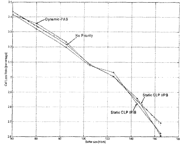
Figure 7 - Aggregate Cell Loss Ratio
